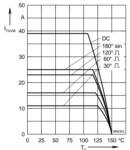
Fig. 9 Maximum forward current at case temperature
